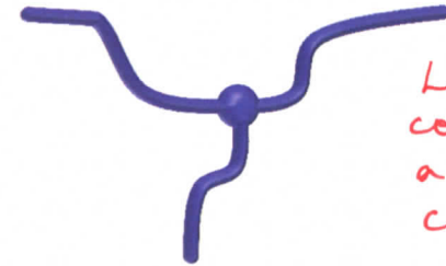
Star Polymer
