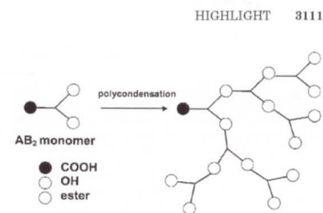
Figure 1. AB 2 polycondensation as described by Flory 5 leads to a hyperbranched macromolecule.
