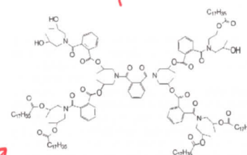
Figure 4. A typical structure of a Hybrane* macromolecule, built up from phthalic anhydride and an excess of diisopropanol amine; the OH end groups are partly esterified with stearic acid. This product is being tested for plastics additives applications.
