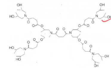
Figure 5. Based on succinic anhydride and diisopropanol amine, this Hybrane* is water soluble, and has been tested, for example, for paper coating applications.
